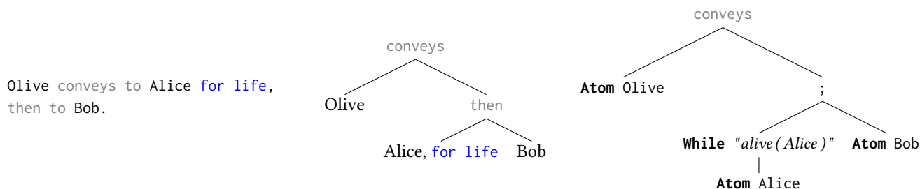
Figure 1. Parsing and desugaring a single conveyance.
